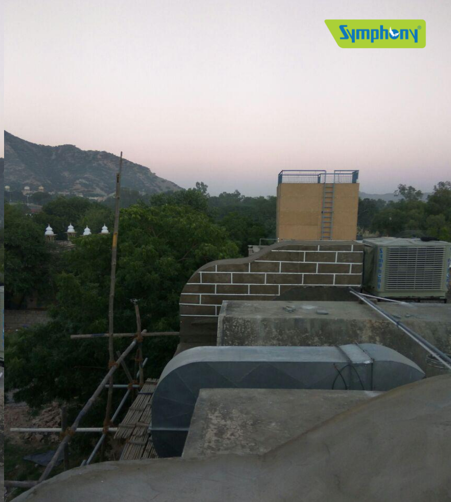
Ducting – All machines are connected to 25 feet duct with direct outlet grill.
